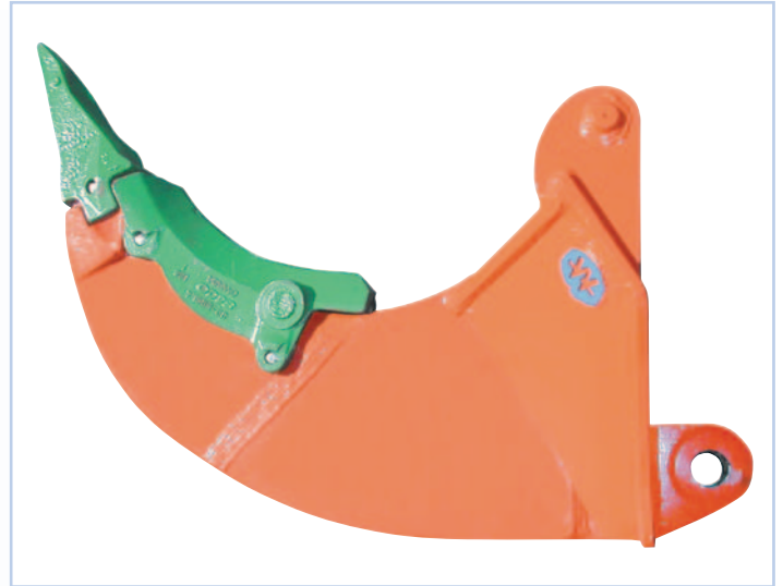
Rock ripper XXHD for extreme conditions, made from WHD 450 special wear steel, exchangeable protective shroud and tooth from Esco
