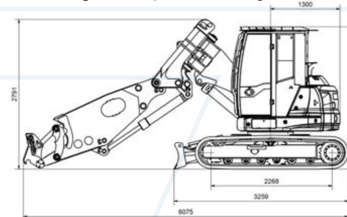
Abmessungen - Transport Blue-/e-Badger
