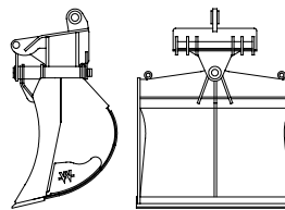
Tiltor V8, Model L30 / L33 / L35 / L43 Excavator: 24-32 / 32-38 / 32-47 / 38-47 to
