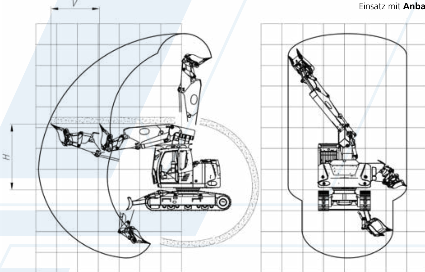
Abmessungen - Transport yellow Fox
