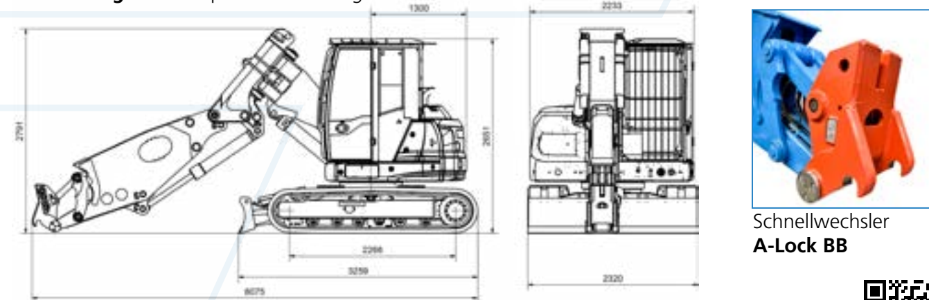
Abmessungen - Transport Blue-/e-Badger
