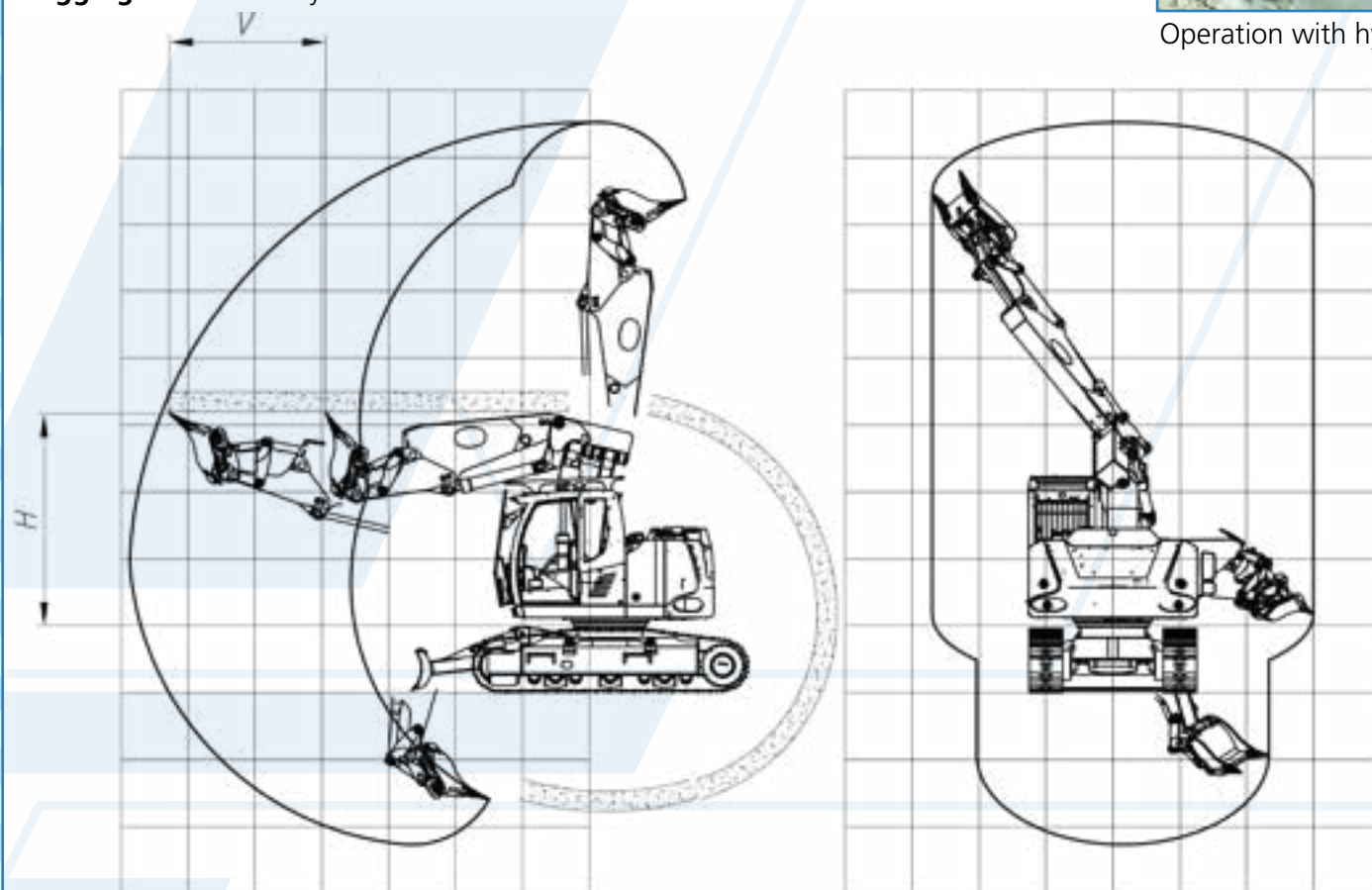
Operation with hydraulic cutter WR18
