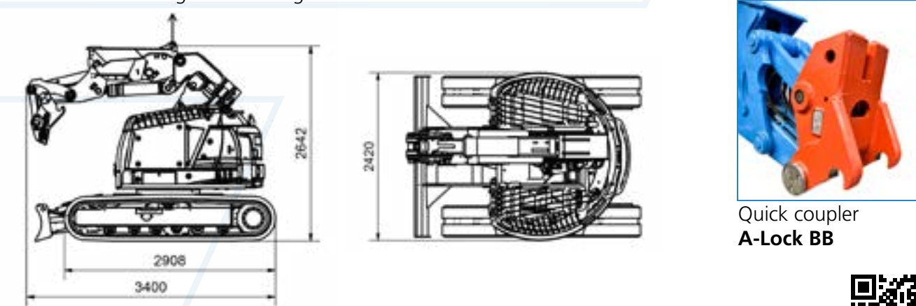
Dimensions - loading mini-/e-Badger
