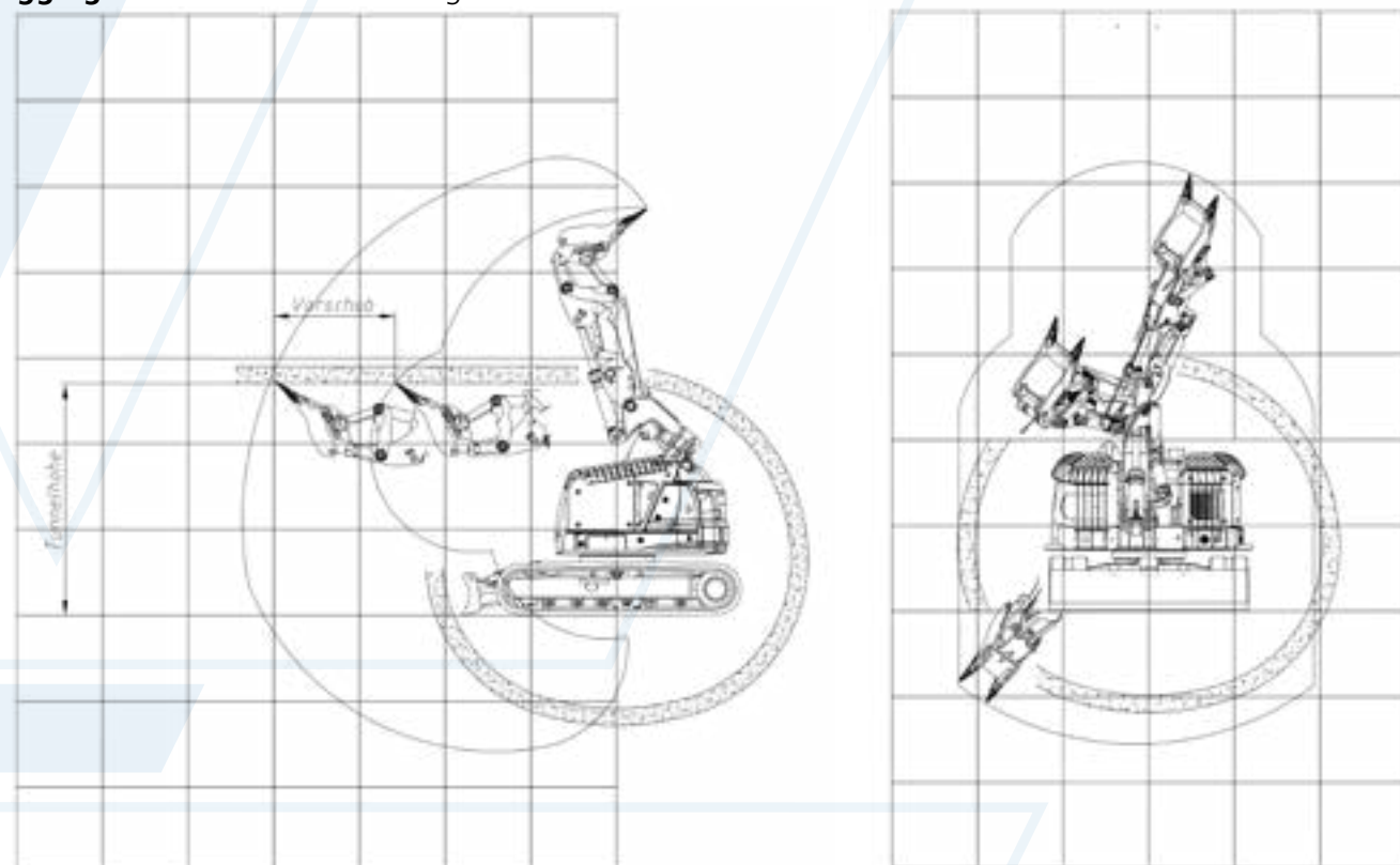
Dimensions - loading mini-/e-Badger
