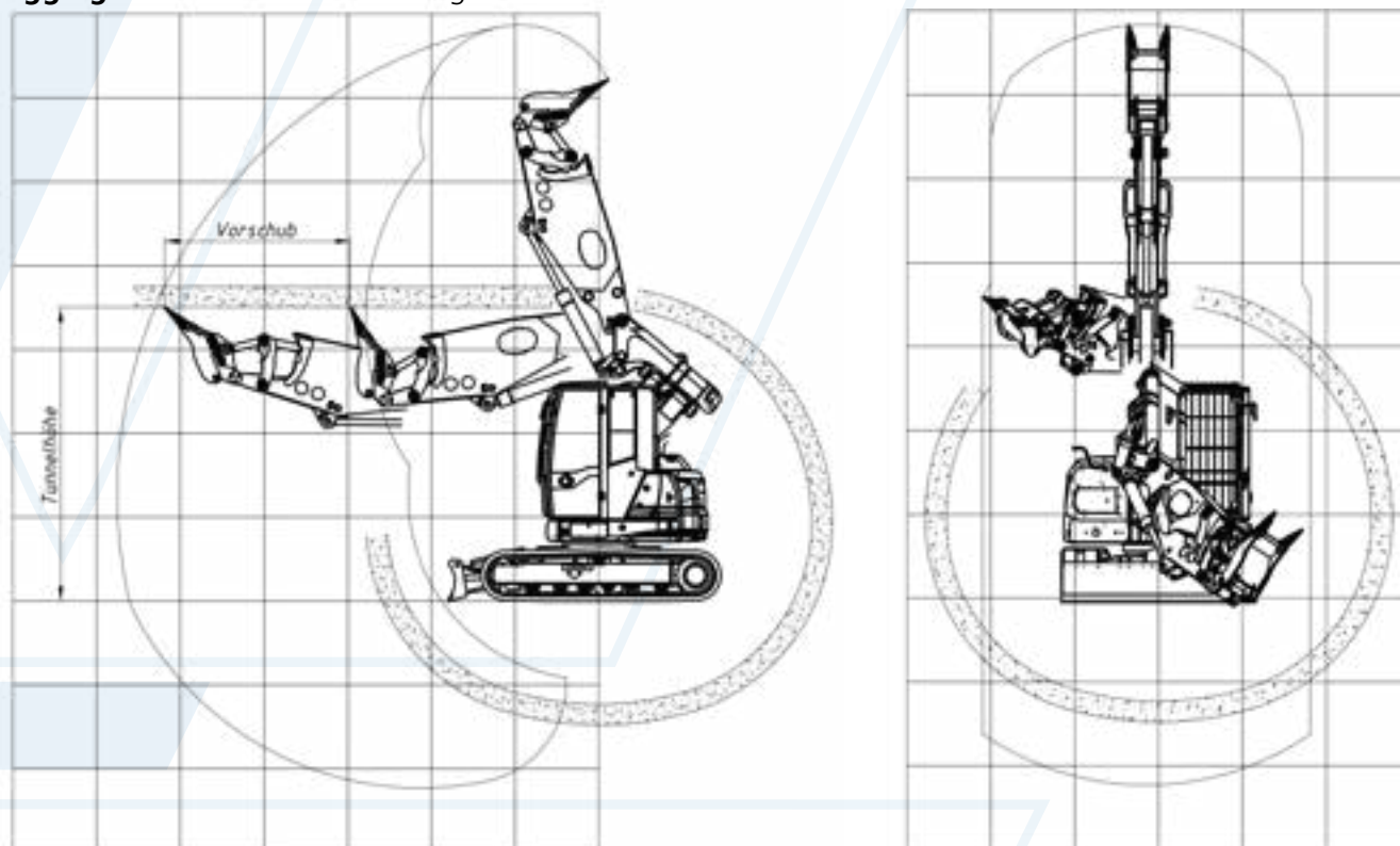
Hydraulic cutter with the e-Badger
